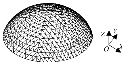
(a) At Node 1 Typical instability modes and their corresponding instability nodes for the spherical shell model.
